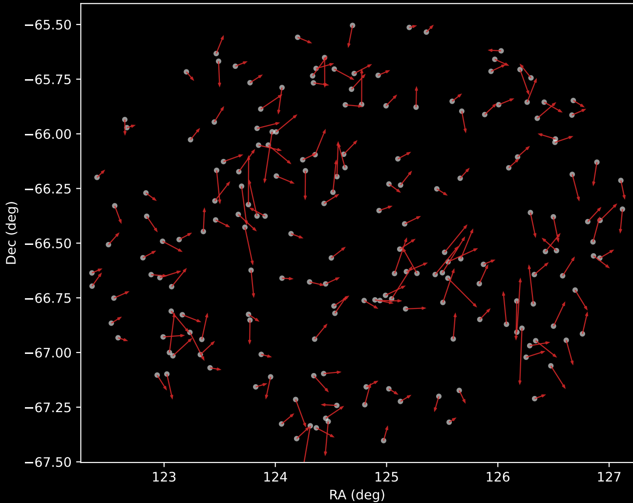
GALAH DR4 Cluster 6 Proper Motion Vectors (n=187)
