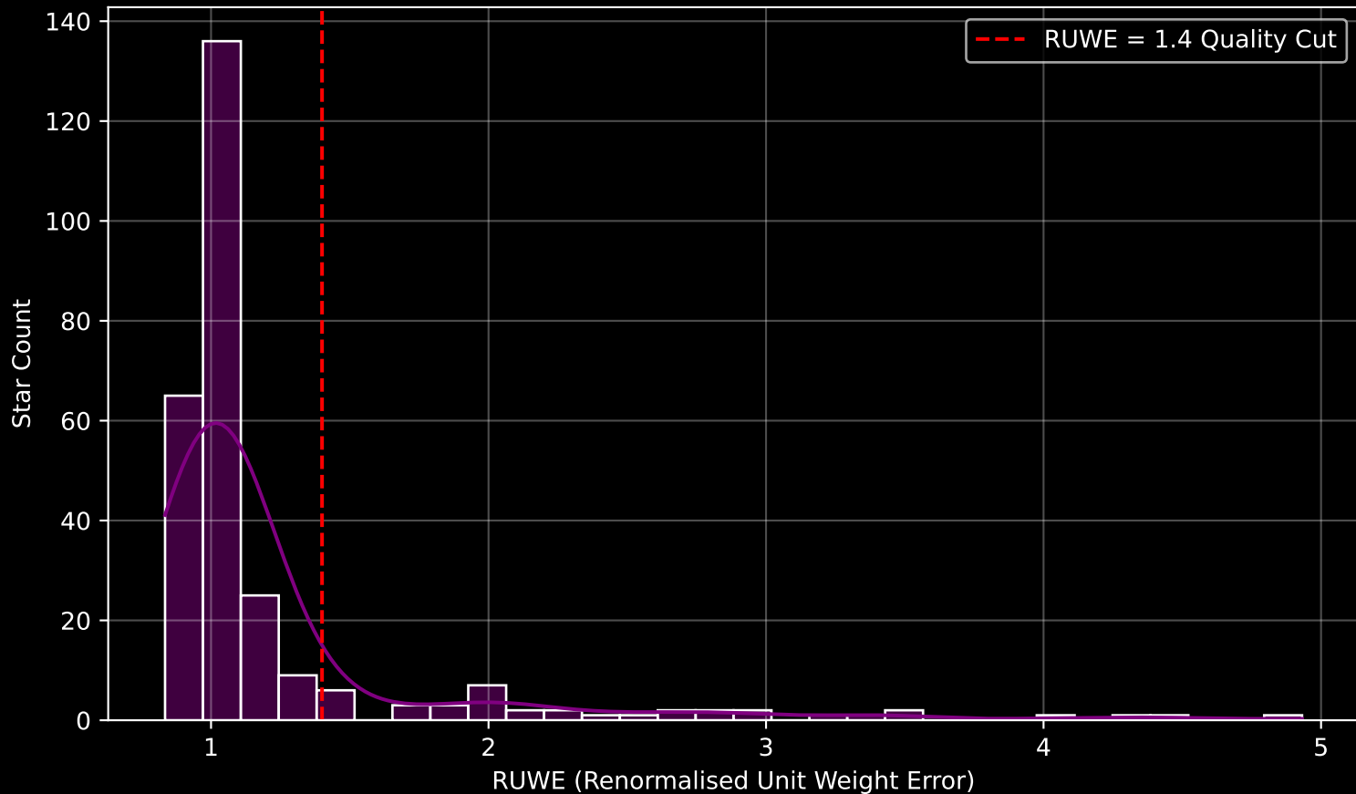
GALAH DR4 Field [7008] RUWE Distribution (n= 274)
