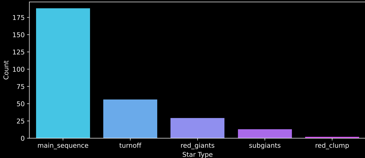
GALAH DR4 Field: [7008] Count plot of Star Type
