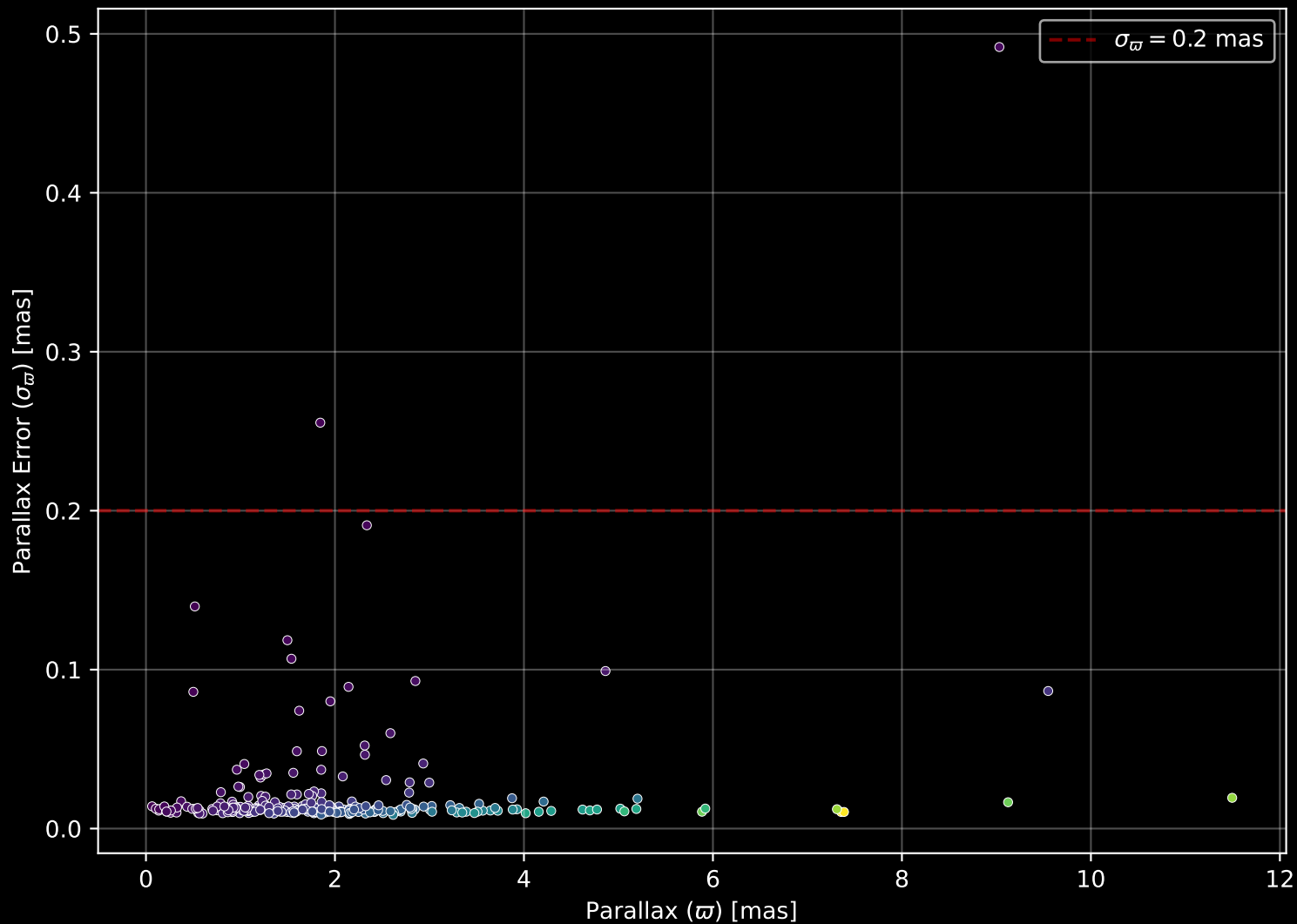
GALAH DR4 Field: [7008] Parallax Quality (n= 288)
