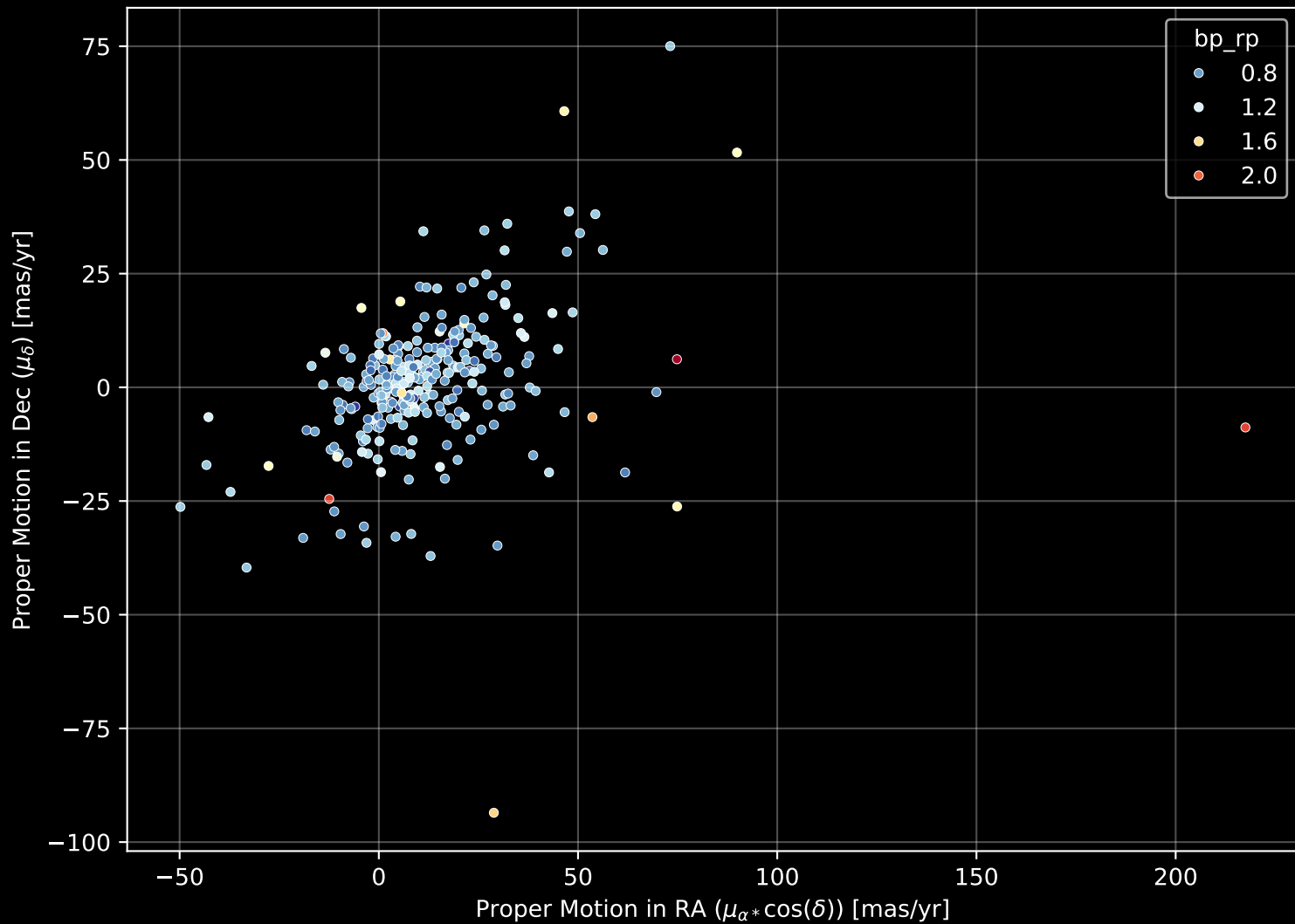
GALAH DR4 Field: [7008] Proper Motion Diagram (n= 288)
